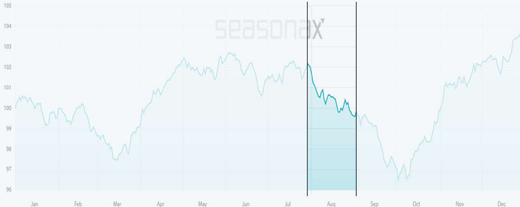
Seasonal Trend of DAX Over 25 Years
